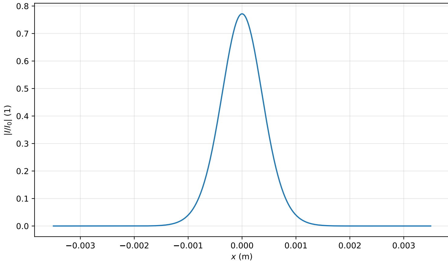
Intensity profile I(x, y = 0, z = 1.592m)/I_0 , P_{in}=0.3P_{cr} , artificial time
